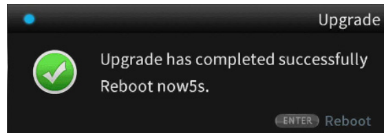
Restart screen
